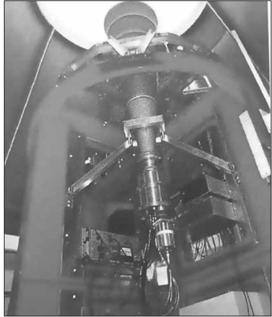
Fig 3.2: 20GHz liquid-helium-cooled receiver front-end under development at Jodrell Bank Radio Observatory. (Photograph: J Fielding 2004)
